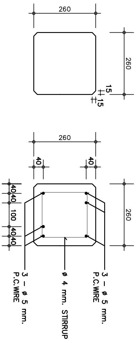
SECTION (A)
