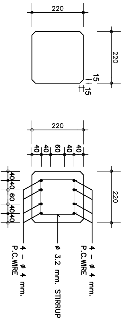
SECTION (A)
