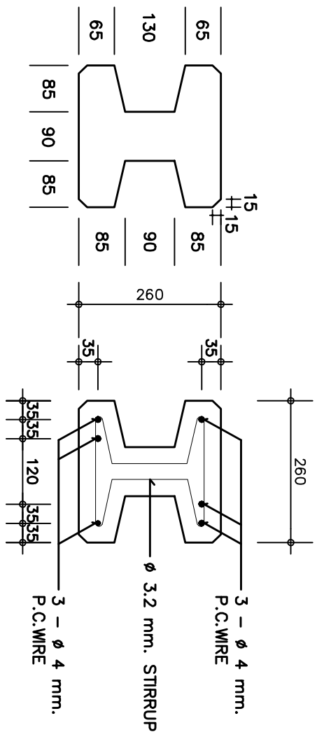
SECTION (A)
